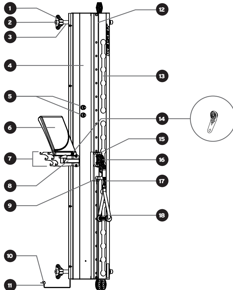
Figure 4. Performance Trainer
