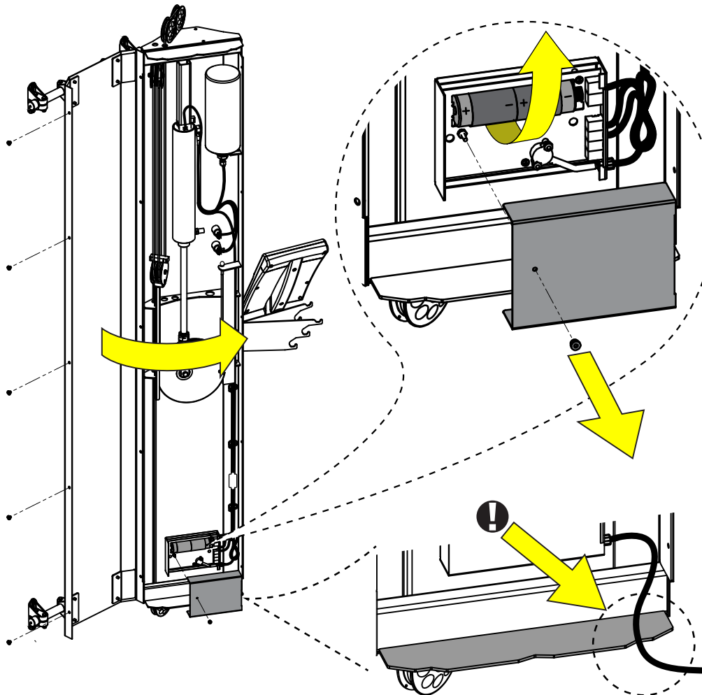
Figure 13. Battery Replacement
