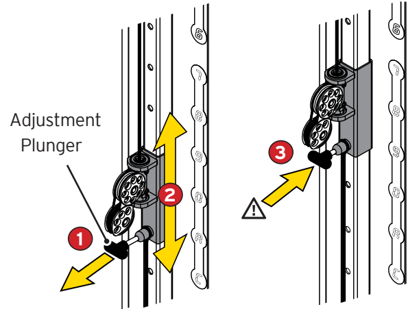
Figure 6. Vertical Adjustment
