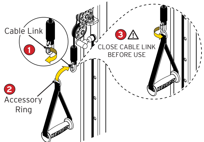
Figure 7. Connecting the Cable Accessory
